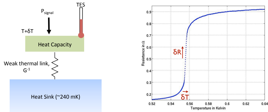
Figure 1-7. Left: Illustration of a thermal circuit for a typical Transition Edge Sensor (TES) detector highlighting the principles of signal detection. A weakly thermally sunk heat capacity absorbs power, P_{\text{signal}} , which is to be measured. Variations in the absorbed power change the heat capacity's temperature, which is measured by a TES operating under strong electro-thermal feedback. Right: Plot of resistance versus temperature for a typical TES illustrating the principles of negative electro-thermal feedback [77]. The TES is voltage biased into the middle of its superconducting-to-normal transition. Small changes in the TES temperature produce large changes in the TES resistance. Since the TES is voltage biased, an increase (or decrease) in the temperature produces an increase (or decrease) in the resistance leading to a decrease (or increase) in the Joule heating power supplied by the bias. This canceling effect corresponds to a strong negative electro-thermal feedback making the current through the TES nearly proportional to P_{\text{signal}} .
