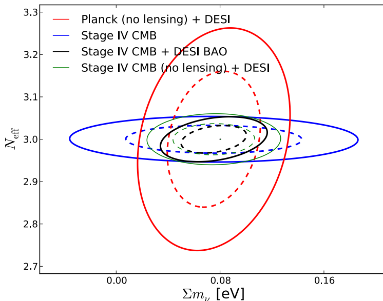
Figure 1-4. The same as Figure 1-3, but showing forecasts for a model including effective number of neutrino species on the plane \Sigma m_\nu - N_{\text{eff}} plane. A Stage-IV CMB experiment will not be able to distinguish between the standard model value of N_{\text{eff}} = 3.046 and the integer value of 3 at high statistical significance, but it should be able to prefer one over the other at the \sim 2\sigma level.
