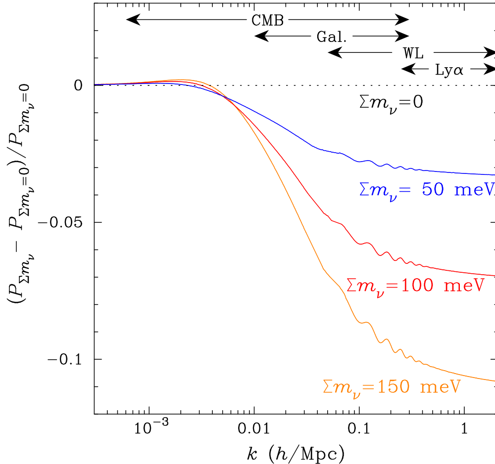
Figure 1-1. Neutrino mass suppresses the matter density power spectrum due to free streaming below the matter-radiation equality scale. The shape of the suppression is highly characteristic and precision observations over a range of scales can measure the sum of neutrino masses (here assumed all to be in a single mass eigenstate). Also shown are the approximate ranges of experimental sensitivity in the power spectrum for representative probes: the cosmic microwave background (CMB), galaxy surveys (Gal.), weak lensing of galaxies (WL), and the Lyman-alpha forest (Ly \alpha ). The CMB lensing power spectrum involves (an integral over) this same power spectrum, and so is also sensitive to neutrino mass.
