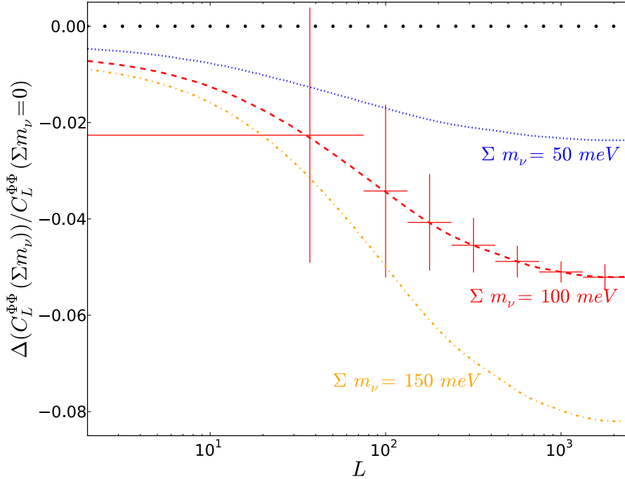
Figure 1-5. The effect of massive neutrinos on the CMB lensing potential power spectrum C_L^{\Phi\Phi} . The fractional change in C_L^{\Phi\Phi} for a given value of \sum m_\nu is shown relative to the case for zero neutrino mass. Projected constraints on C_L^{\Phi\Phi} for a Stage-IV CMB experiment are shown for \sum m_\nu = 100 meV. Here we have approximated all of the neutrino mass to be in one mass eigenstate and fixed the total \Omega_m h^2 and H_0 . The 1\sigma constraint for \sum m_\nu is approximately 45 meV for lensing alone and drops to 16 meV when combined with other probes.
