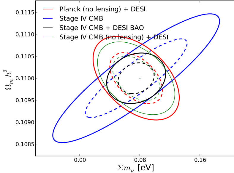
Figure 1-3. Forecasted 1\sigma and 2\sigma constraints in the \Sigma m_\nu - \Omega_m h^2 plane showing the synergy of an experiment like DESI and a Stage-IV CMB lensing experiment. For contrast, a combination of Planck data with the lensing information removed and DESI are shown in the red contours. The blue contours show the constraint generated by the CMB lensing experiment, corresponding to a 24 meV constraint on massive neutrinos. The black contours show the result of adding only DESI BAO information, resulting in a 16 meV constraint. This can be compared to the case where no Stage-IV CMB lensing information but all galaxy clustering information is used, yielding a 24 meV constraint. The combination of a Stage-IV CMB experiment and BAO information from DESI should allow a robust measurement of the sum of the neutrino masses.
