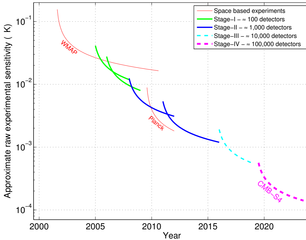
Figure 1-6. Plot illustrating the evolution of the raw sensitivity of CMB experiments, which scales as the total number of bolometers. Ground-based CMB experiments are classified into Stages with Stage II experiments having O(1000) detectors, Stage III experiments having O(10,000) detectors, and a Stage IV experiment (such as CMB-S4) having O(100,000) detectors.
