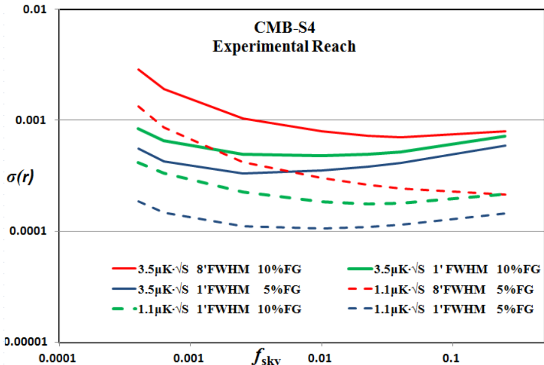
Figure 1-3. Expected statistical uncertainty on tensor-to-scalar ratio for a few Stage-IV CMB configurations, plotted as a function of sky coverage. Forecast for two beam sizes (1' and 8' FWHM) and two overall sensitivity goals (3.5 and 1.1 \mu\text{K}\cdot\sqrt{\text{s}} ) are displayed. Foregrounds are assumed to be cleaned to 10% or 5% residual level (in map). We find the stated goal of \sigma(r) < 10^{-3} is achieved or exceeded.
