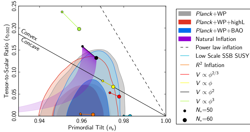
Figure 1-1. Current CMB constraints on the combined n_s - r parameter space [22].
