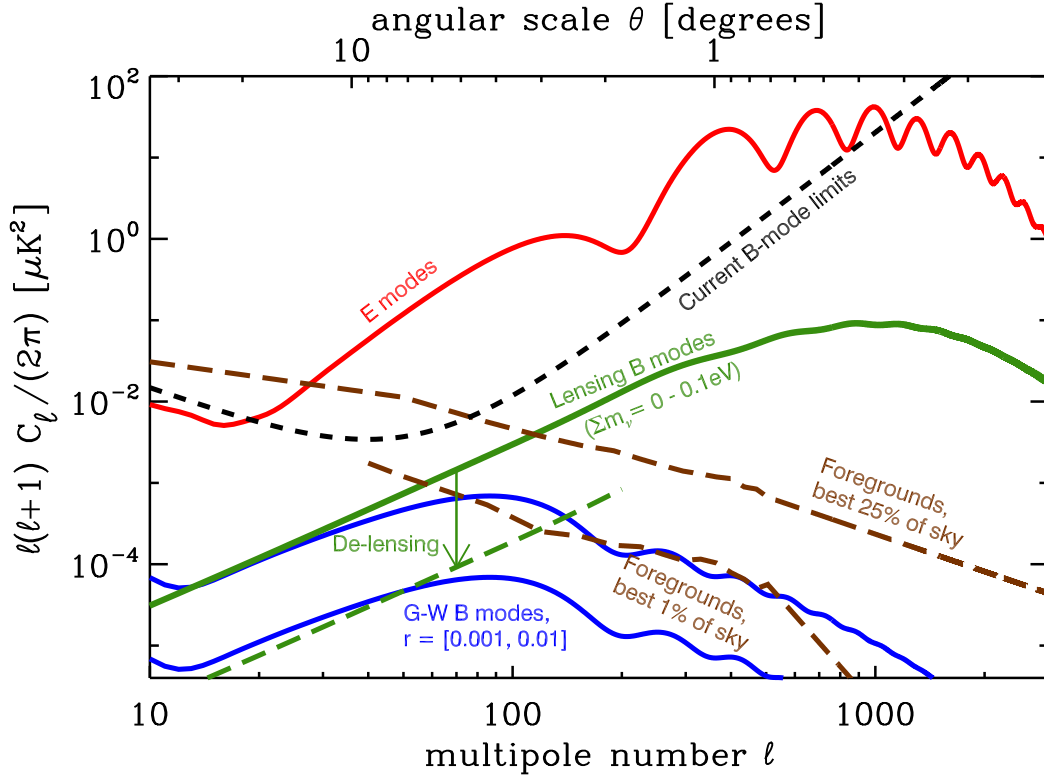
Figure 1-2. Expected signal levels for the E -mode (red, solid), inflationary gravitational-wave B -mode (blue, solid), and lensing B -mode (green, solid) signals. The gravitational-wave B -mode signals are shown for tensor-to-scalar ratios of r = 0.001 (the Stage-IV goal) and r = 0.01 (the boundary between small-field and large-field inflation models). The lensing B -mode signal is shown as a band encompassing the predicted signal for values of the sum of neutrino masses 0 \leq \sum m_\nu \leq 0.1\text{eV} . Delensing by a factor of 4 in amplitude is shown schematically by the green arrow, with the residual signal at \ell \leq 200 (where the delensing is critical to the constraint on r ) shown by the green, long-dashed line. The black, short-dashed line shows the level of current 95% upper limits on B modes from WMAP at the largest scales, the BICEP experiment at degree scales, and the QUIET and QUAD experiments at smaller scales. The brown, long-dashed lines show the expected polarized foreground contamination at 95 GHz for the cleanest 1% and 25% of the sky.
