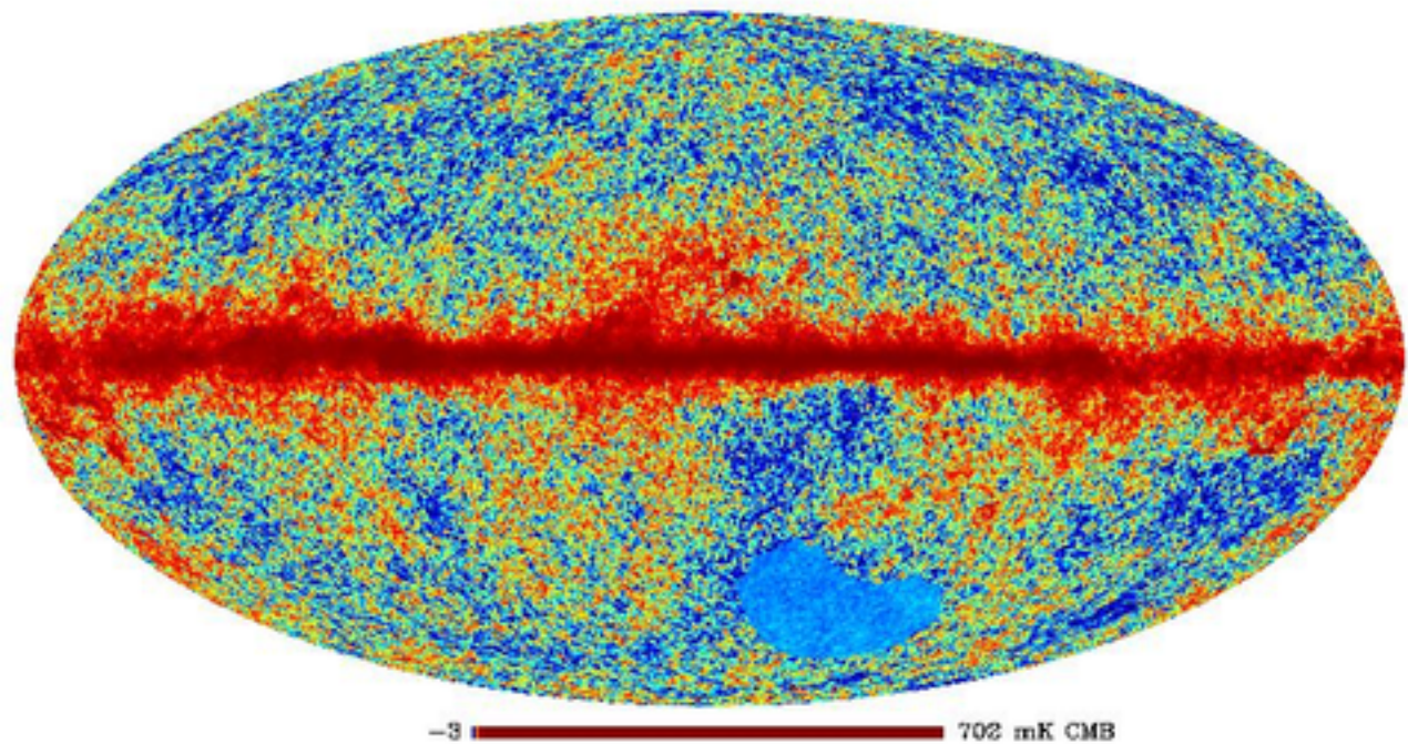
Planck 143 GHz in the field of view of bicep2 T
