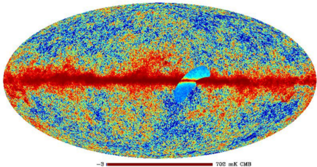
Planck 143 GHz in the field of view of keck T
